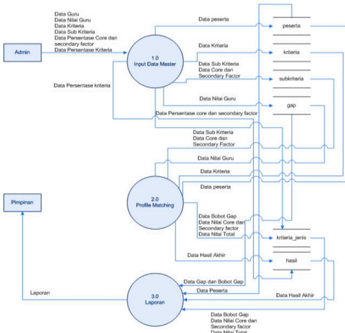
Gambar 5. Diagram level 0
