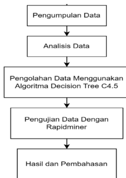
Gambar 1. Metode Penelitian
